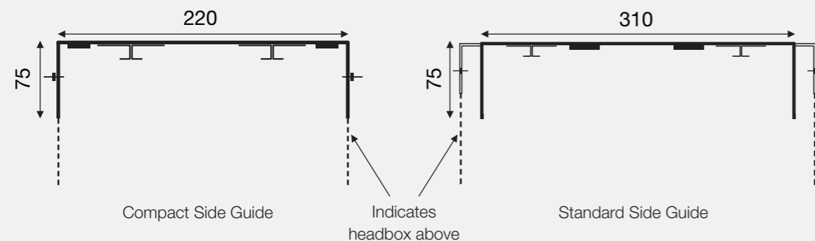
Plan View of Side Guide
